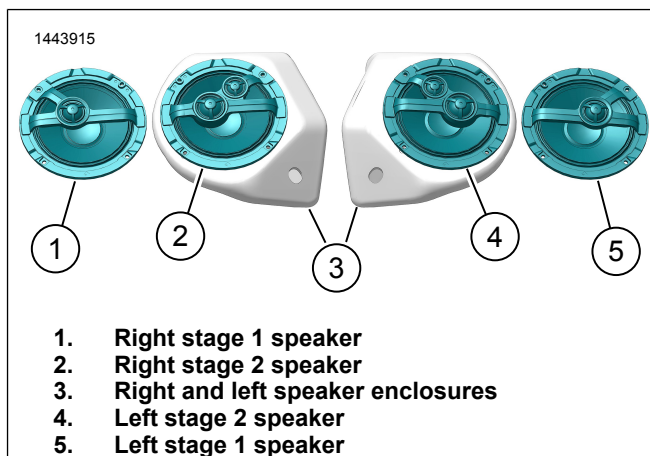
Figure 1. Tour-Pak Speaker Orientation
