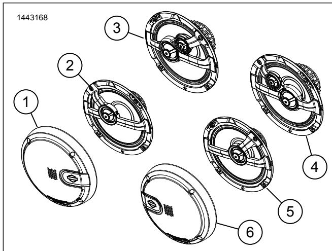
Figure 9. Service Parts, Boom! Audio 6.5 in Rear Speaker Kit
