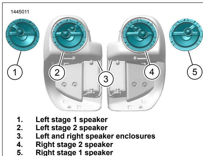
Figure 2. Air Cooled Speaker Orientation
