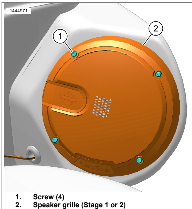
Figure 3. Speaker Pod Grille (Left Side Shown)
