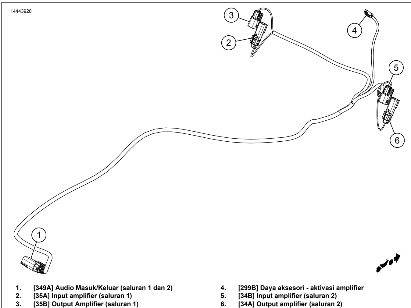
Gambar 3. Harness Speaker Fairing
