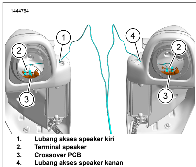
Gambar 1. Harness Kabel Speaker
