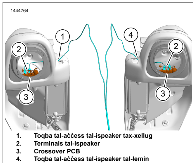
Figura 1. Harness tal-Wajer tal-Ispeaker
