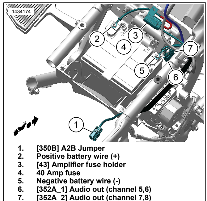
Figure 18. External Wire Harness Routing (Typical)
