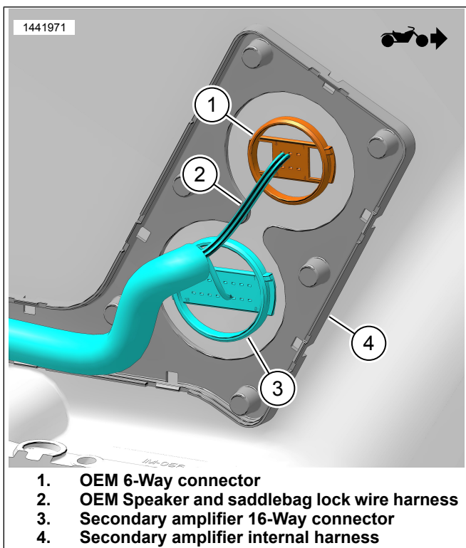
Figure 7. Secondary Amplifier Internal Harness (Inside Saddlebag)
