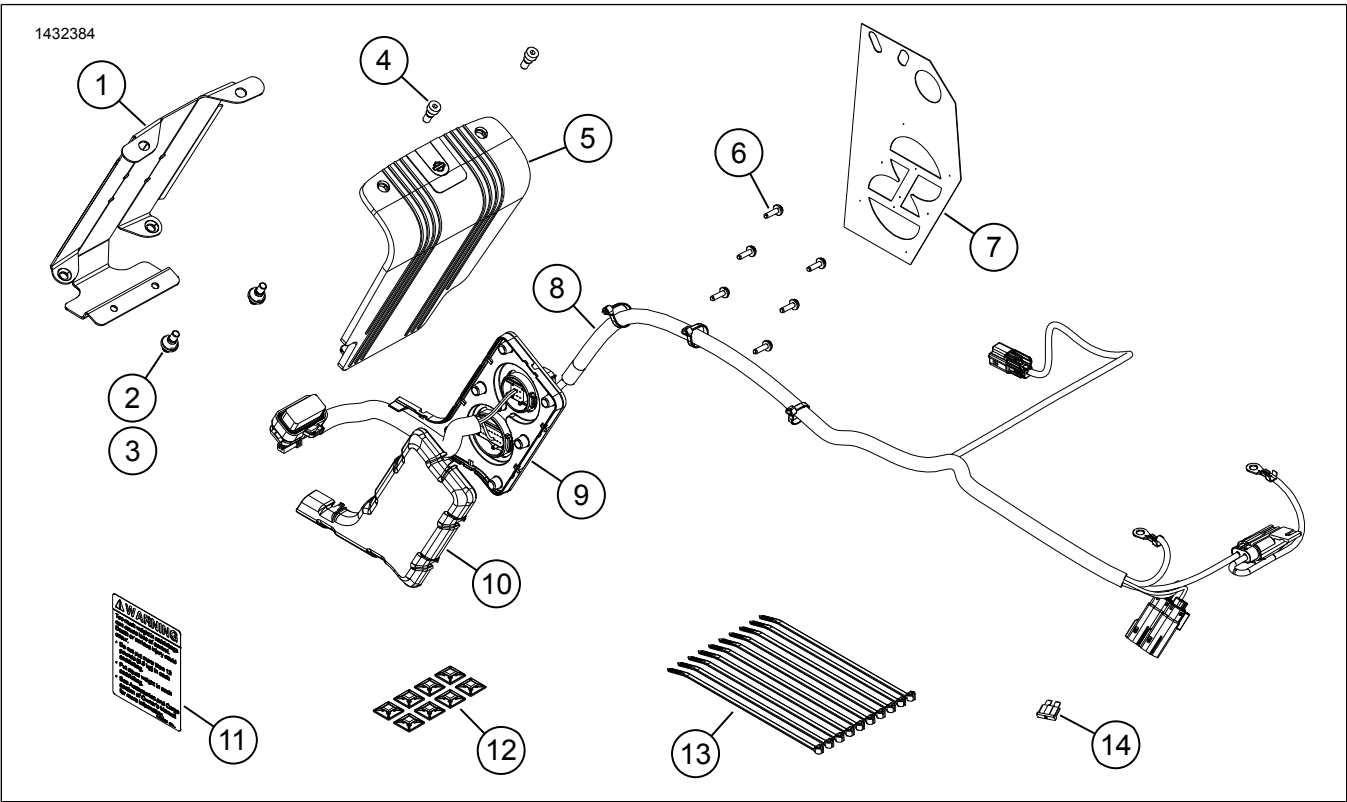
Figure 1. Service Parts: Secondary Amplifier Kit
