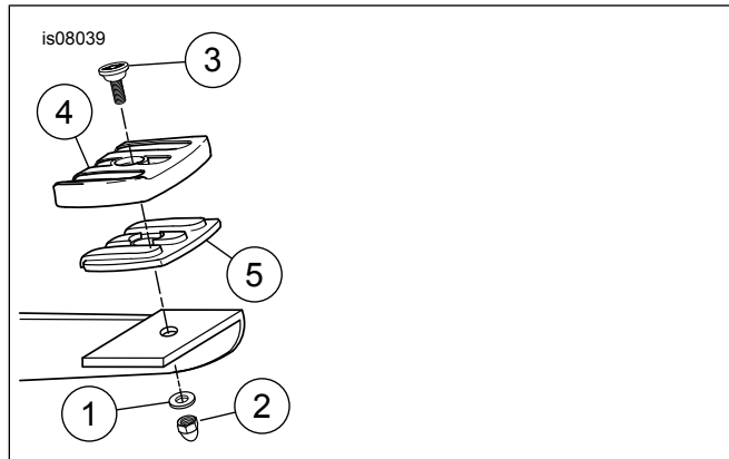
Figure 1. Service Parts
