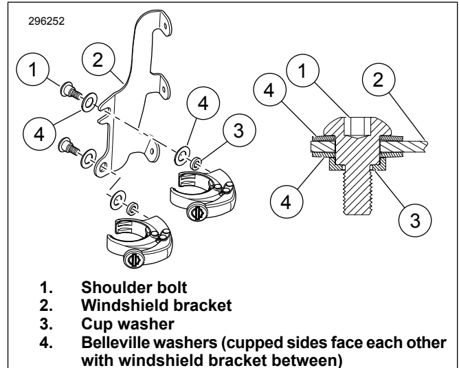
Figure 1. Windshield Mounting Clamp
