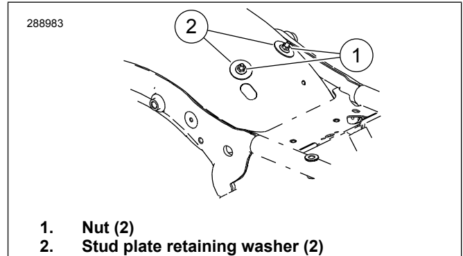
Figure 1. Remove Nuts
