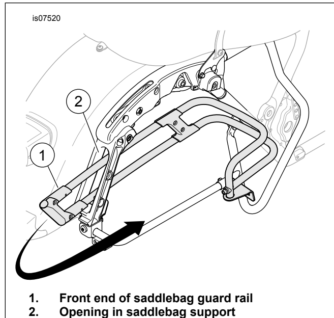
Figure 1. Installation Routing
