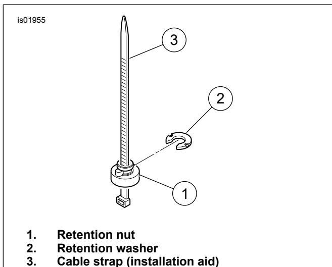
Figure 2. Retention Nut Installation
