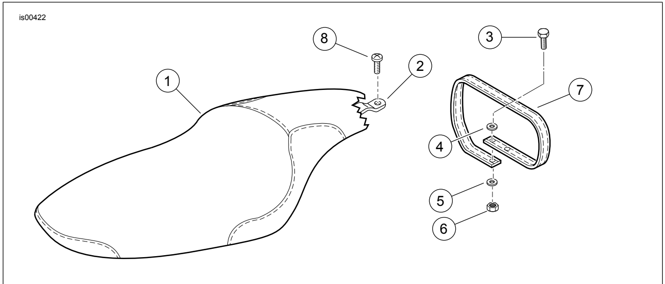
Figure 4. Service Parts: Softail Seats
