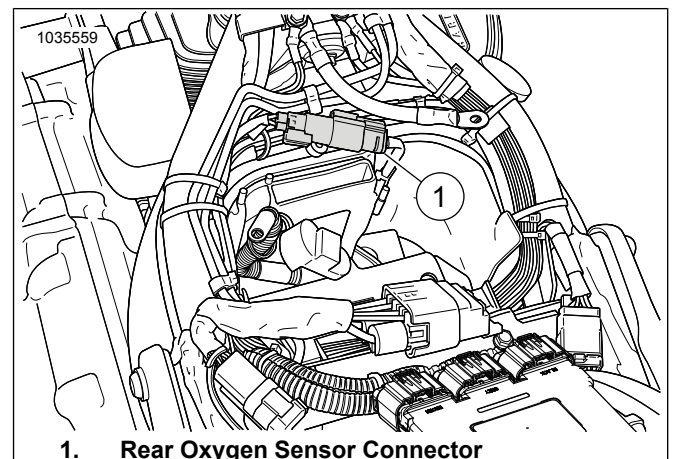
Figure 31. Rear Oxygen Sensor Location
