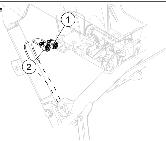
Figure 1. Front and Rear Oxygen Sensor Location
