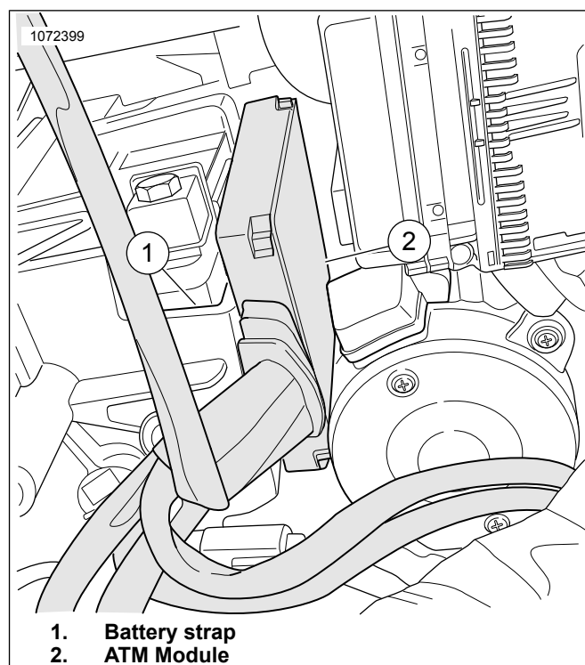
Figure 18. Position Module
