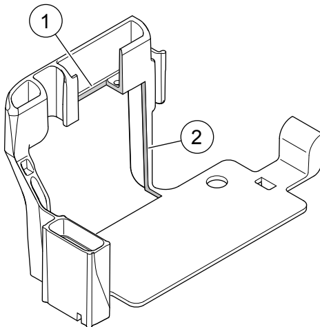
Figure 28. Areas Highlighted To Be Cut Away
