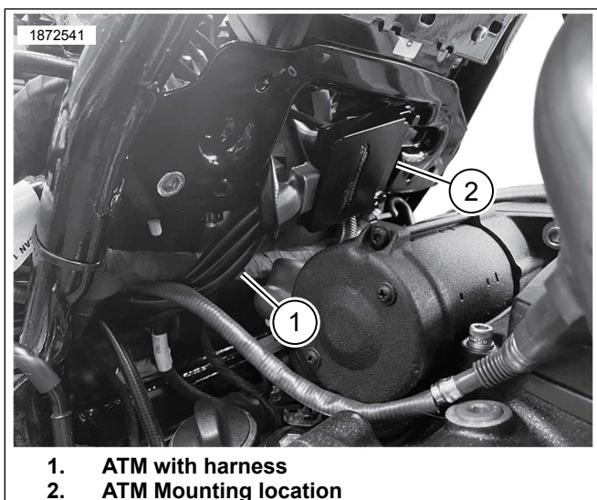
Figure 5. ATM Mounting Location
