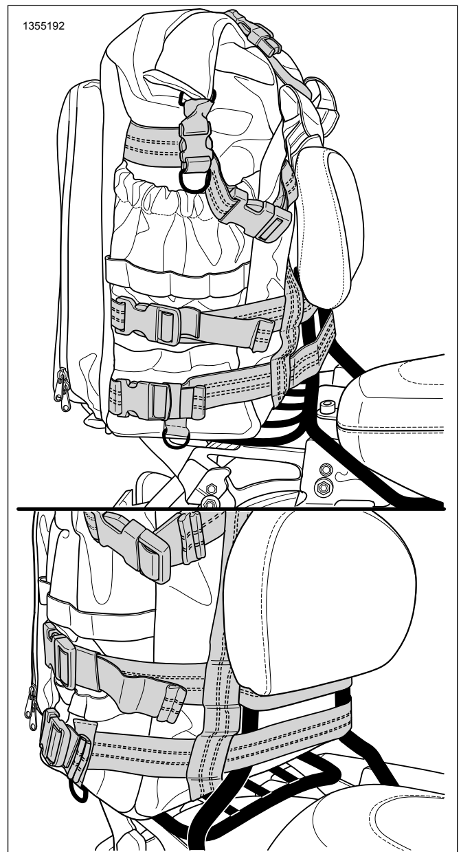
Figure 8. Attachment to Sissybar
