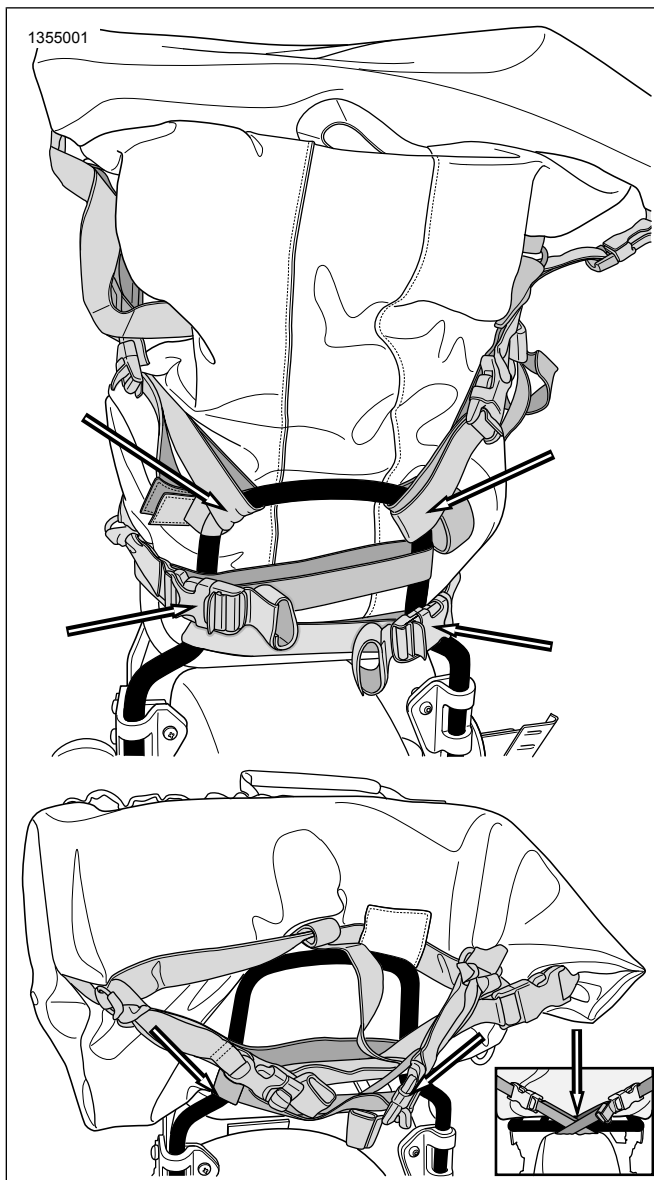
Figure 7. Attachment to Luggage Rack
