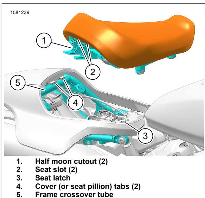
Figure 2. Seat Installation
