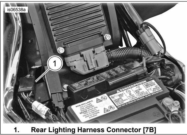
Figure 1. Rear Lighting Harness Connector - Softail Models
