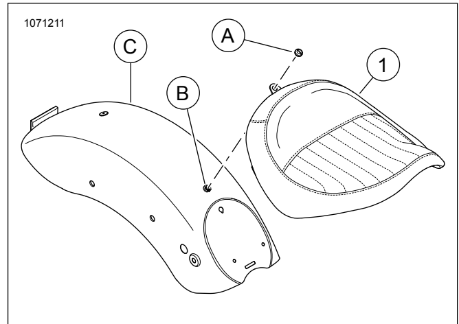
Figure 1. Service Parts: Single post mount
