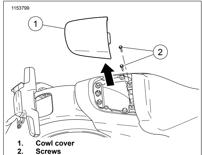
Figure 1. Cowl Cover and Screw Removal
