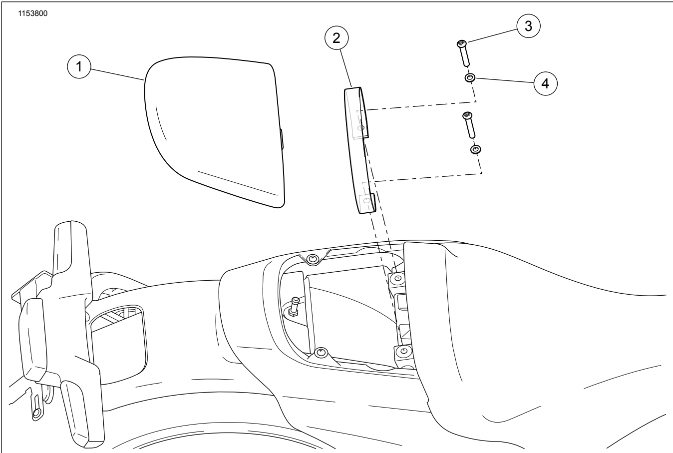
Figure 2. Service Parts: FXDR Passenger Pillion Kit
