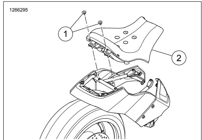
Figure 1. Service Parts: FXDRS Rider Seat
