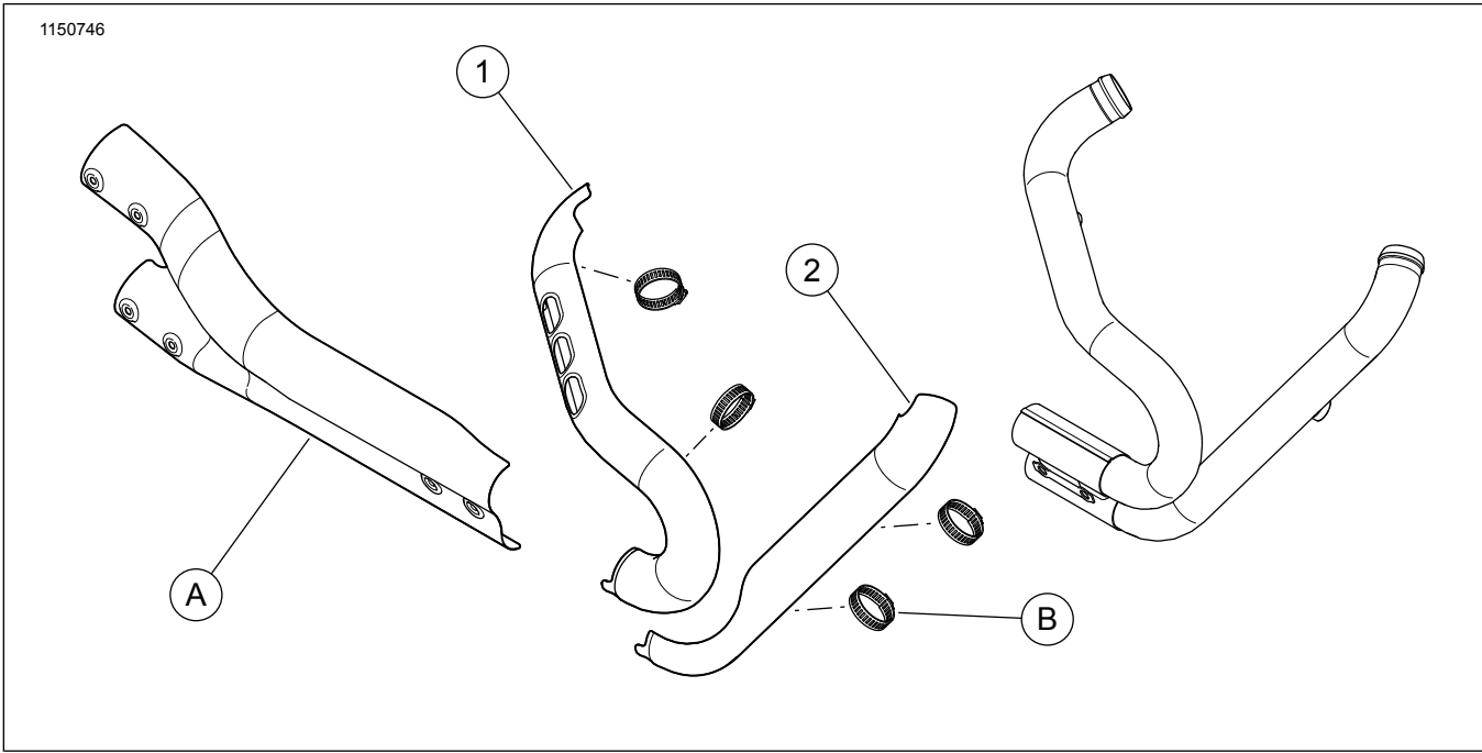
Figure 1. Service Parts: Fat Bob Model Exhaust Shields
