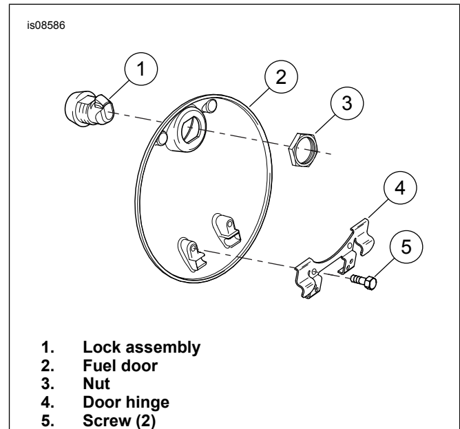
Figure 1. Fuel Door
