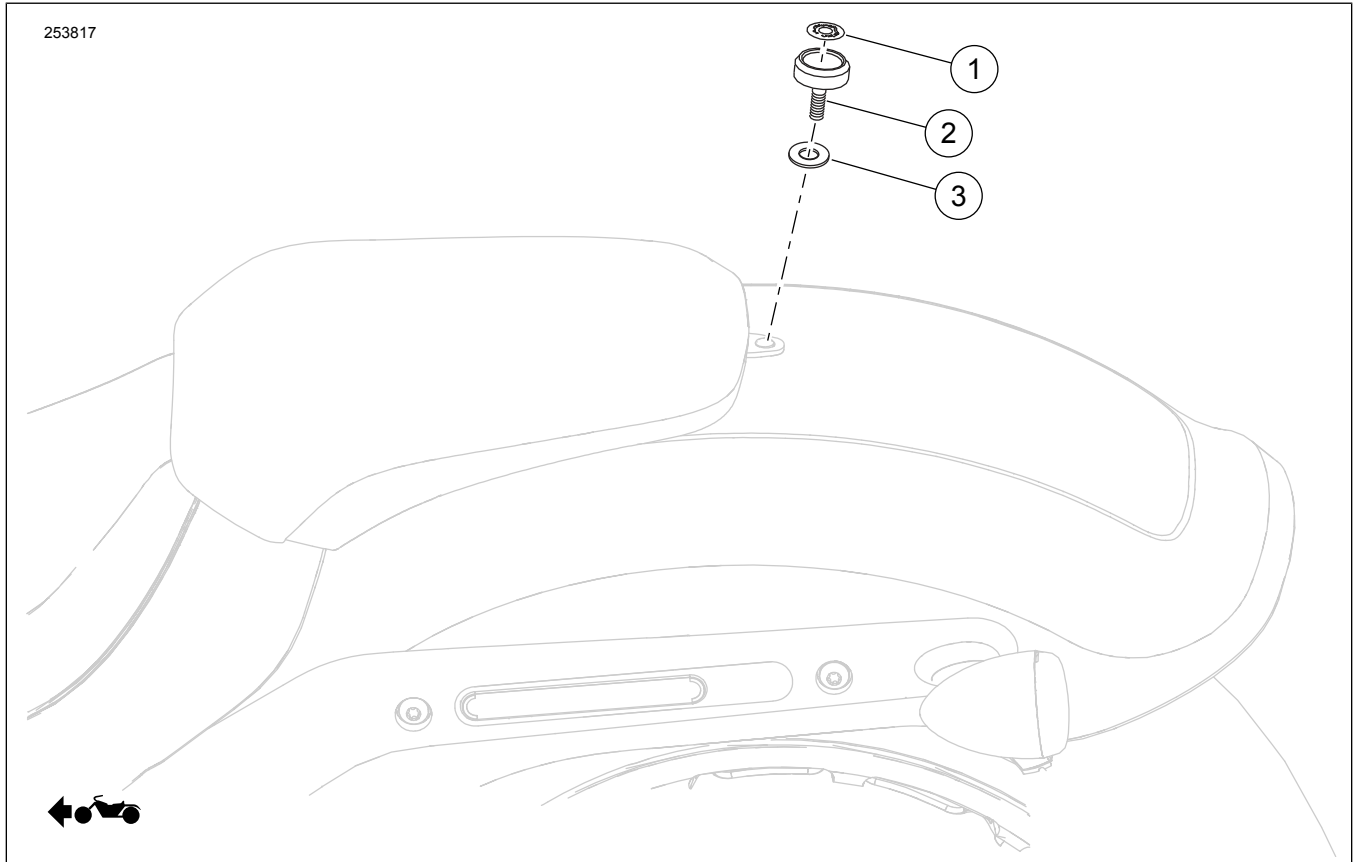
Figure 1. Kit Contents: Rider Backrest Components
