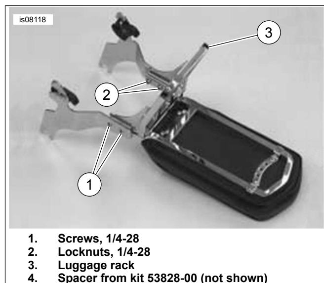
Figure 1. Luggage Rack (shown with detachable sideplates)
