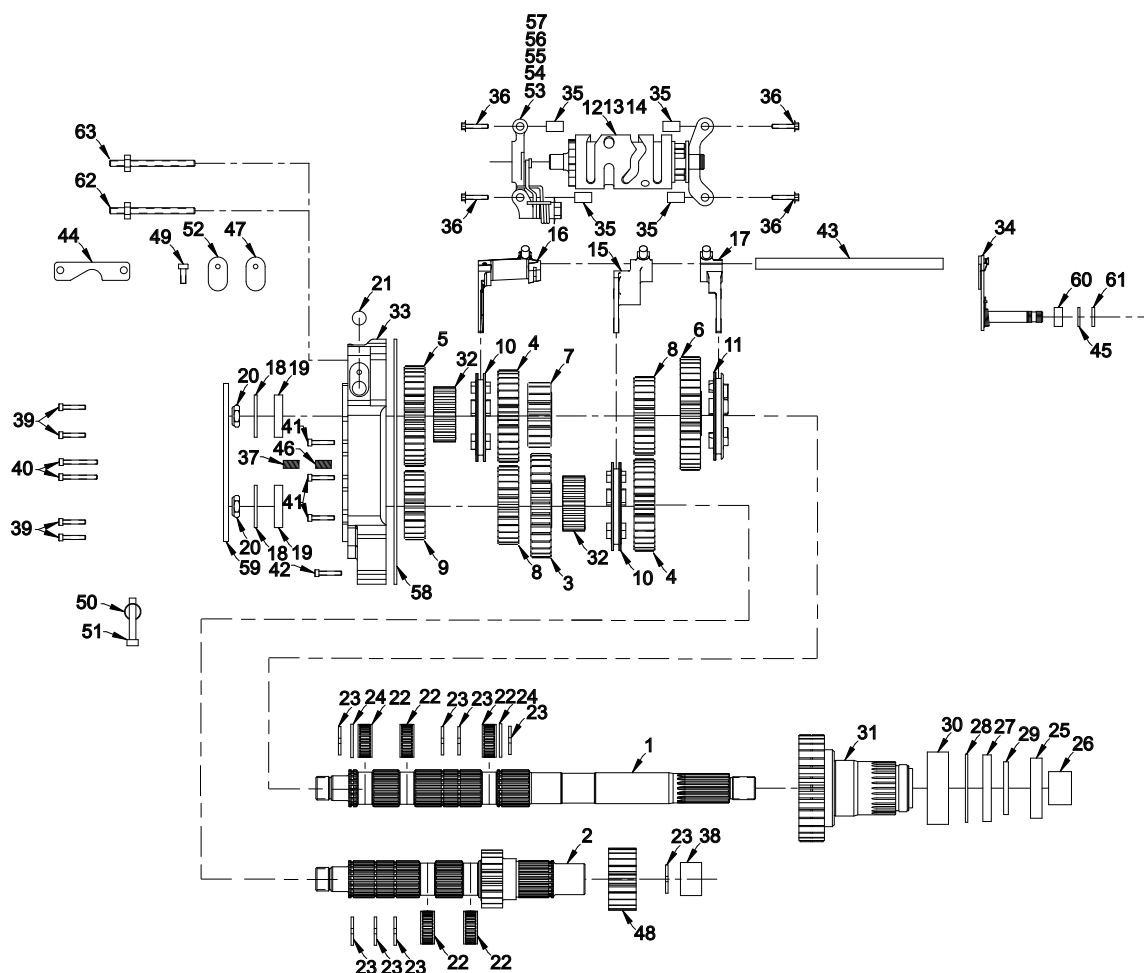
Figure 6. Service Parts: 6 Speed Transmission Super Kit
