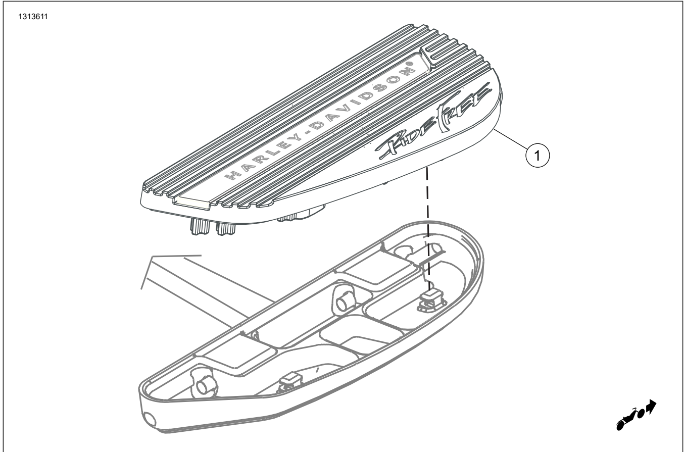
Figure 1. Kit Contents: Footboard Insert Components (Right side shown)
