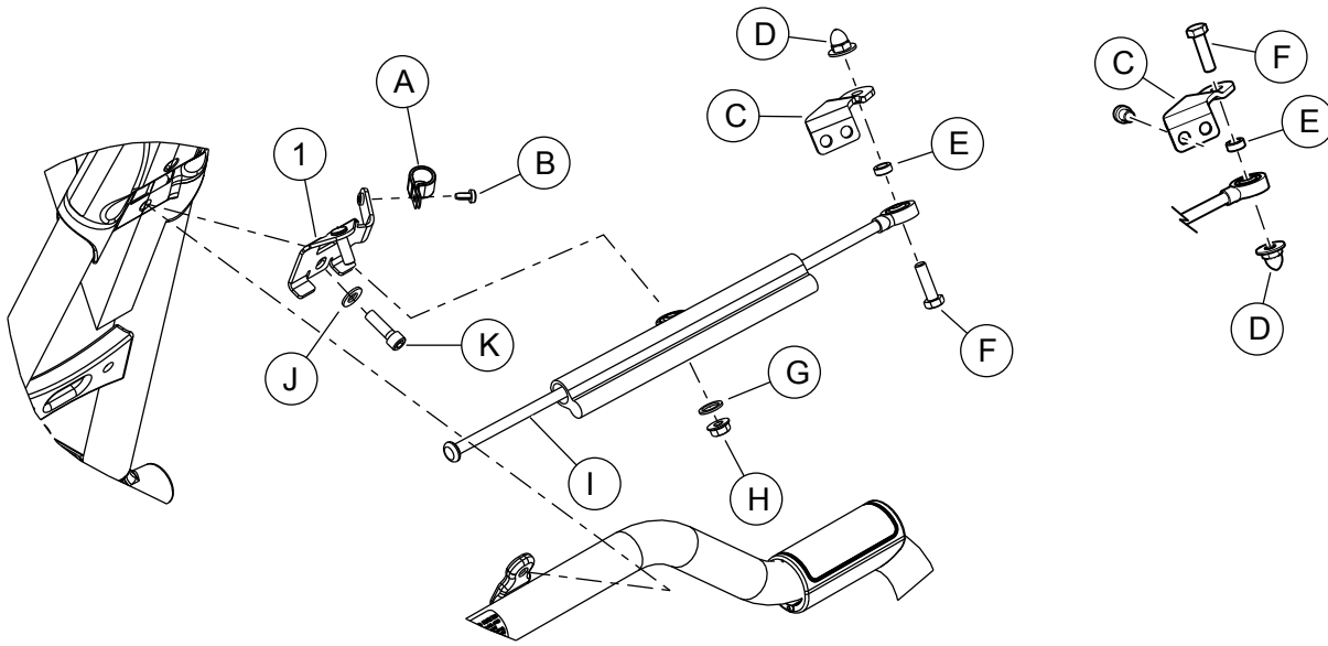
Figure 1. Service Parts: Engine Guard Mounting Bracket Kit
