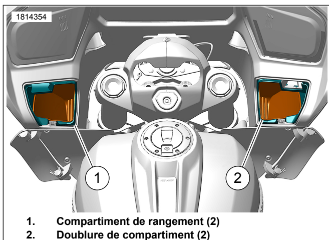
Figure 2. Installer les doublures de compartiment.
