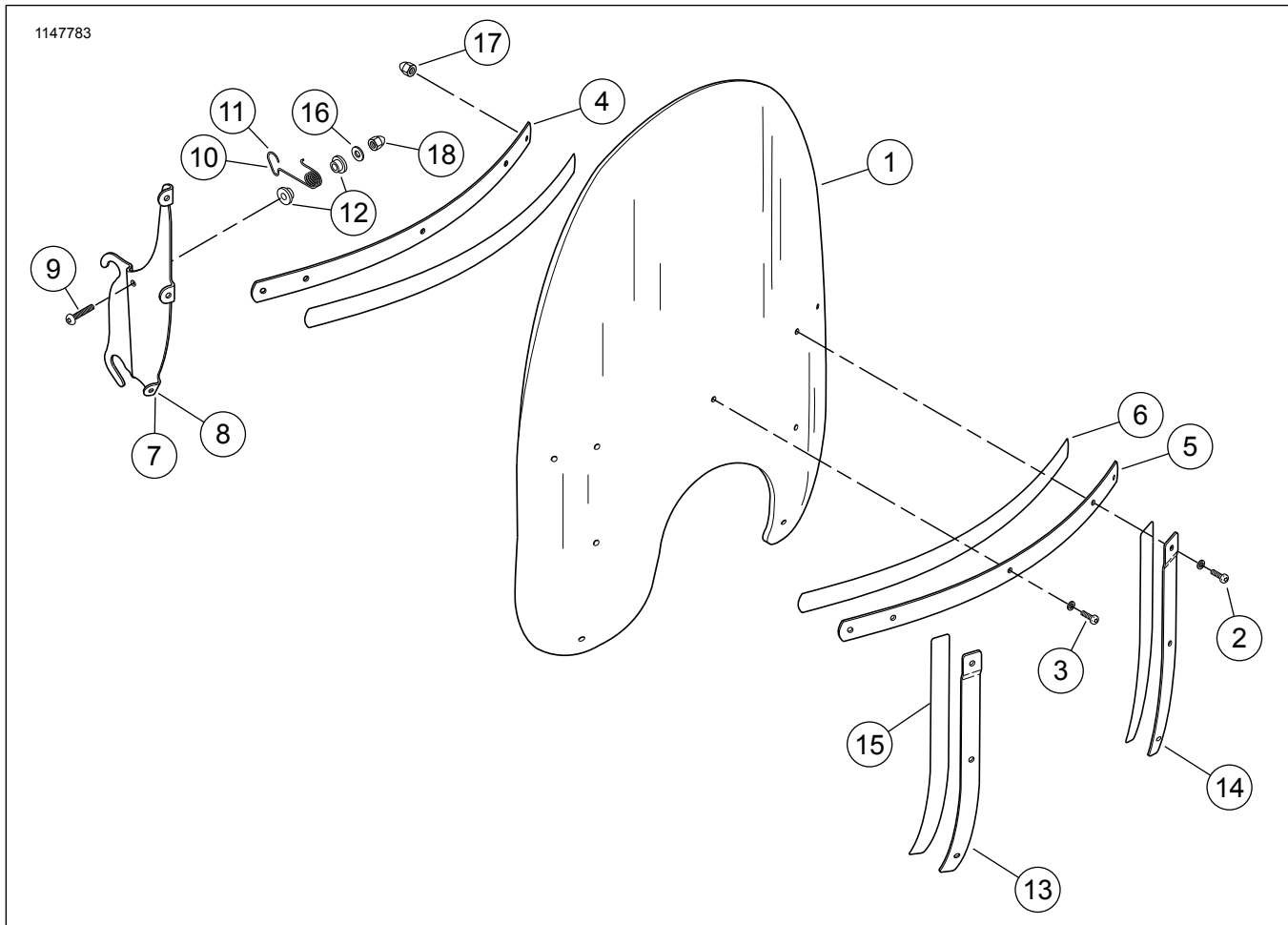
Figura 1. Parts tas-Service: Assemblaġġ tal-Windshield
