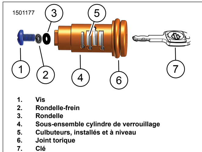
Figure 5. Ensemble verrou assemblé
