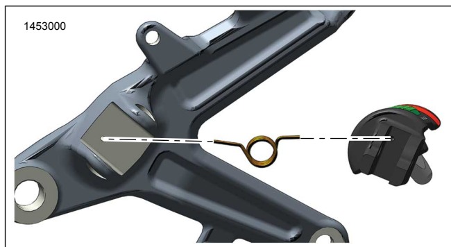
Figure 5. Return Spring Orientation - Kanan
