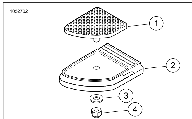
Figur 1. Servicedeler: Sett for liten bremsepedalpute
