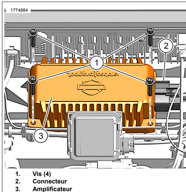
Figure 2. Amplificateur
