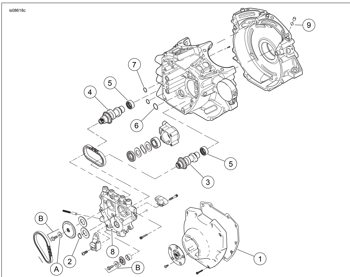
Rajah 3. Bahagian Servis: Kit Penukaran Screamin' Eagle Twin Cam 110 (1800 cc) - Stock Heads
