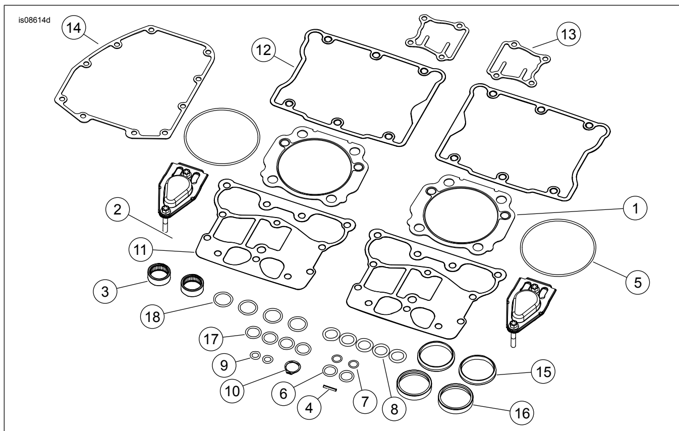
Rajah 4. Bahagian Servis: Kit Penukaran Screamin' Eagle Twin Cam 110 (1800 cc) - Stock Heads
