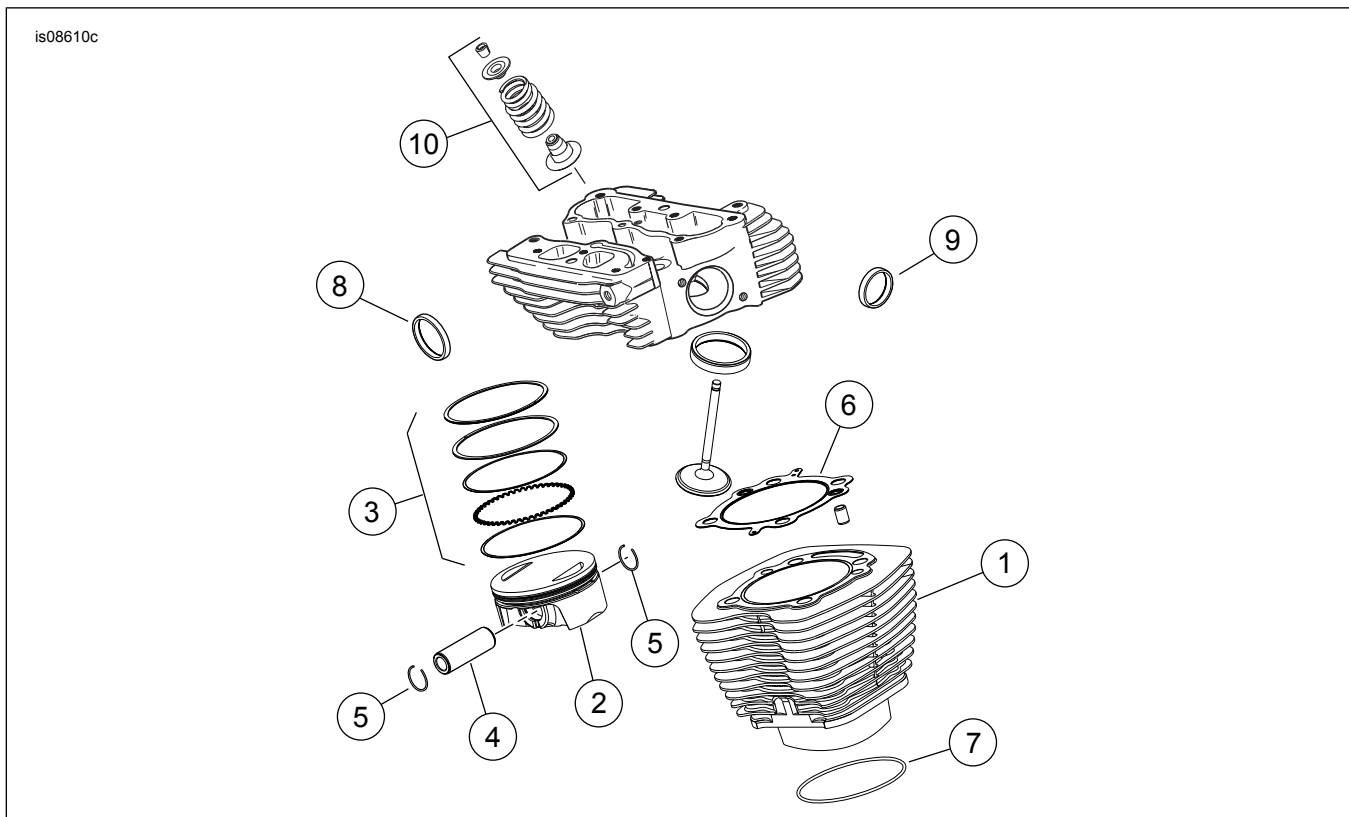
Rajah 1. Bahagian Servis: Kit Penukaran Screamin' Eagle Twin Cam 110 (1800 cc) - Stock Heads
