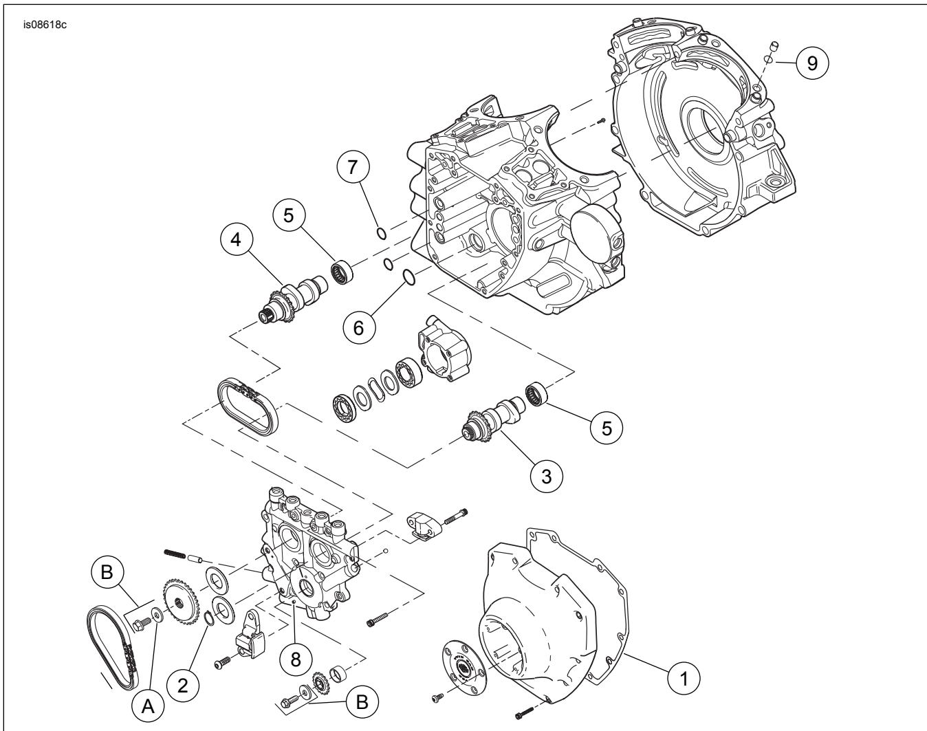
Figure 3. Service Parts: Screamin' Eagle Twin Cam 110 (1800 cc) Conversion Kit - Stock Heads
