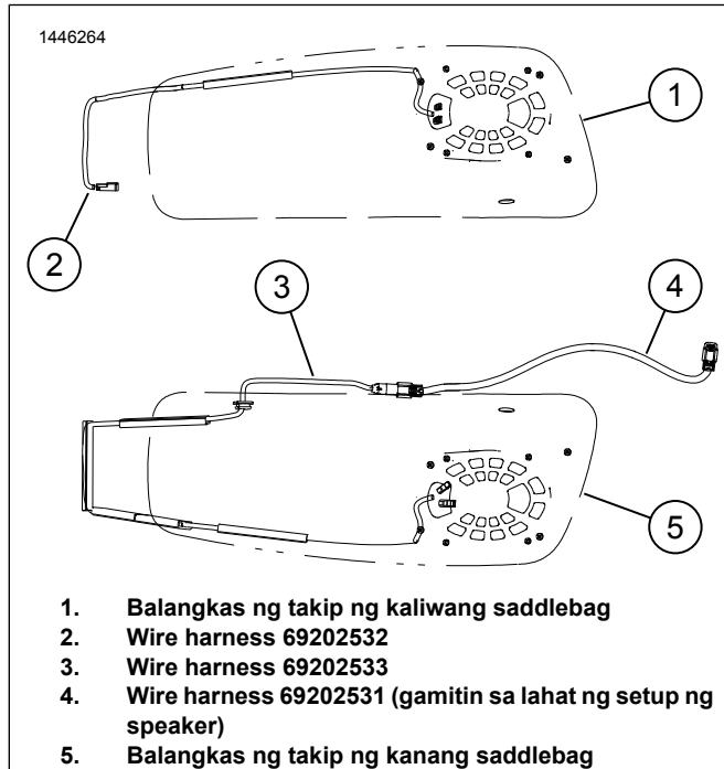
Figure 2. Pag-setup at Pagruruta ng Wire Harness
