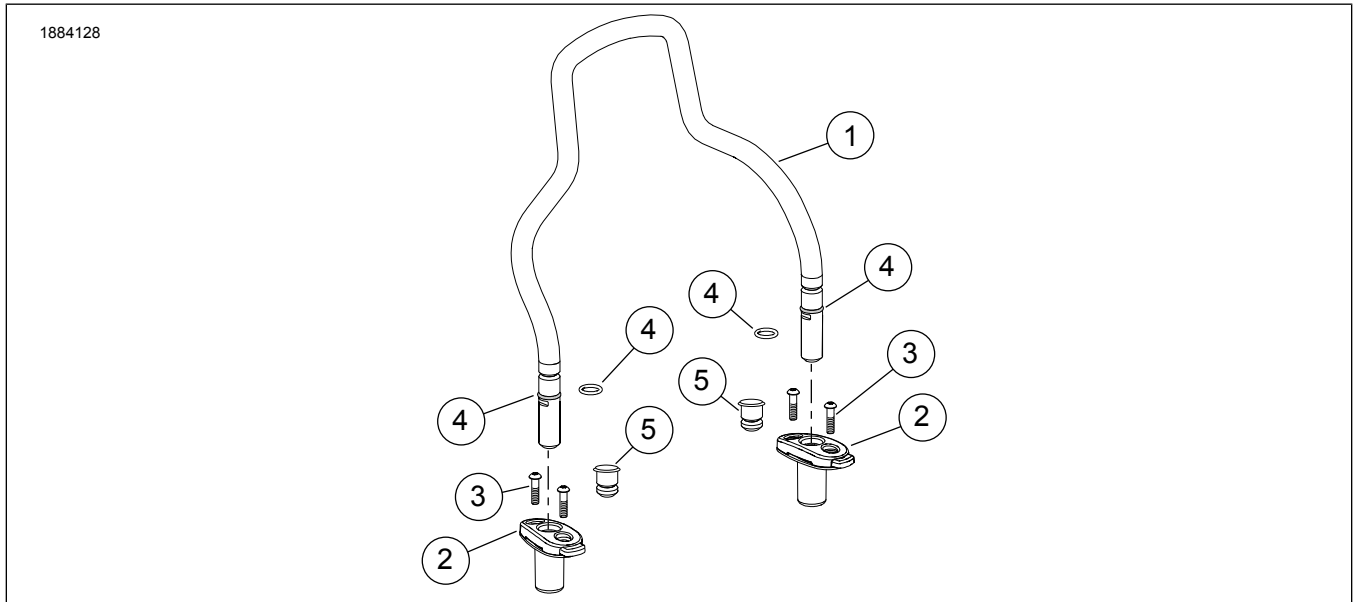
Figure 1. Kit Contents: Quick-Release Sissy Bar Upright Kit
