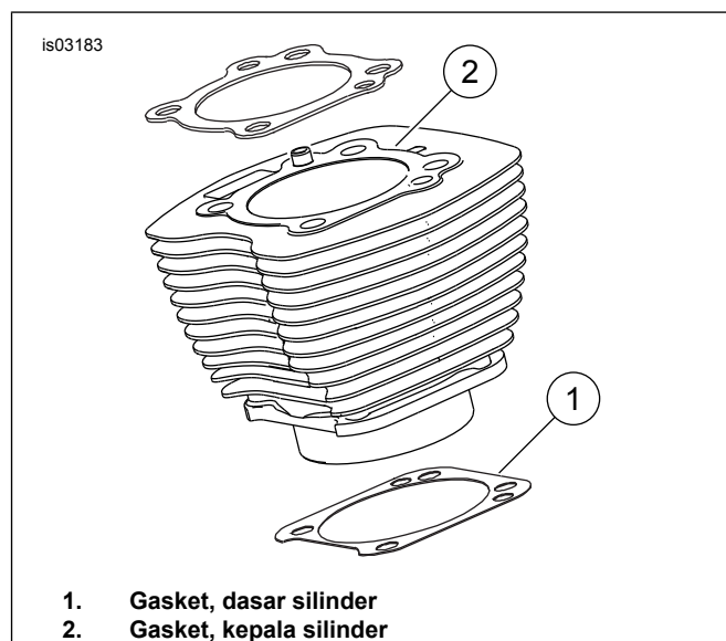
Gambar 1. Gasket Silinder
