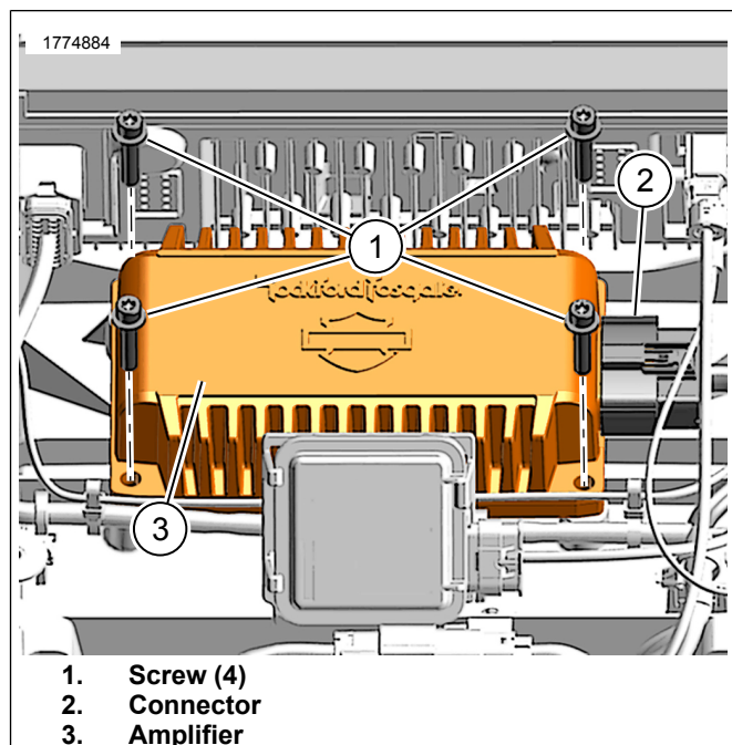
Figure 2. Amplifier
