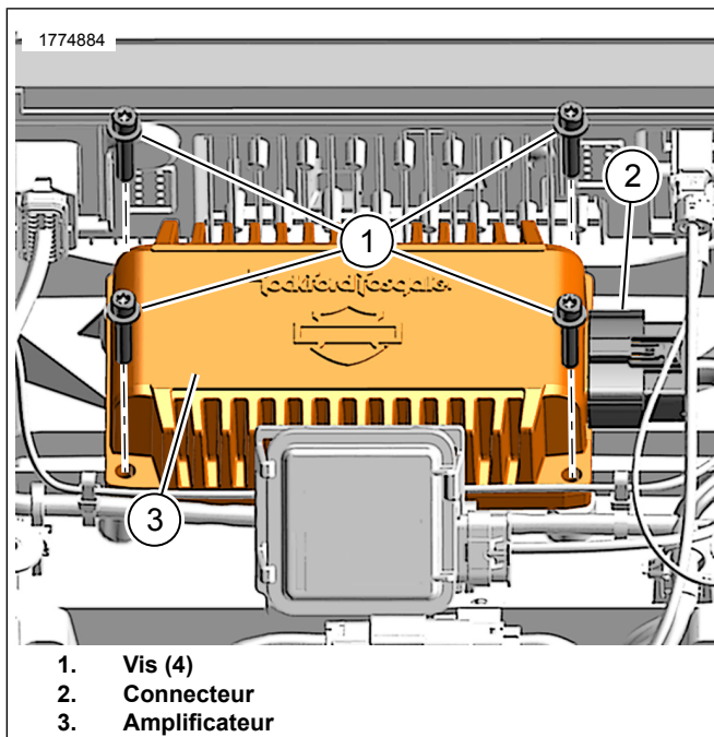
Figure 2. Amplificateur
