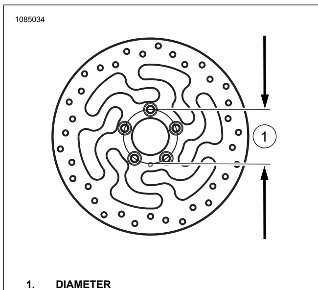
1. DIAMETER Figure 4. Disc Mounting Hole Diameter
