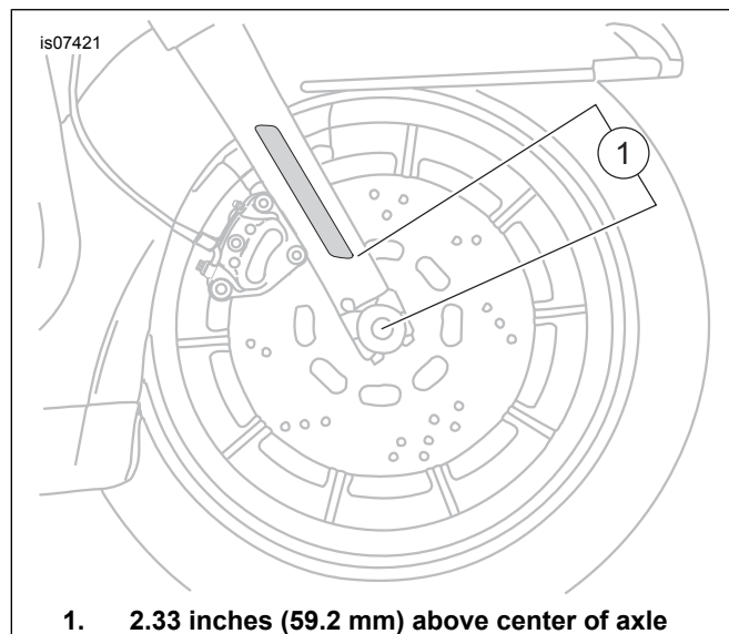
Figure 2. Reflector Placement
