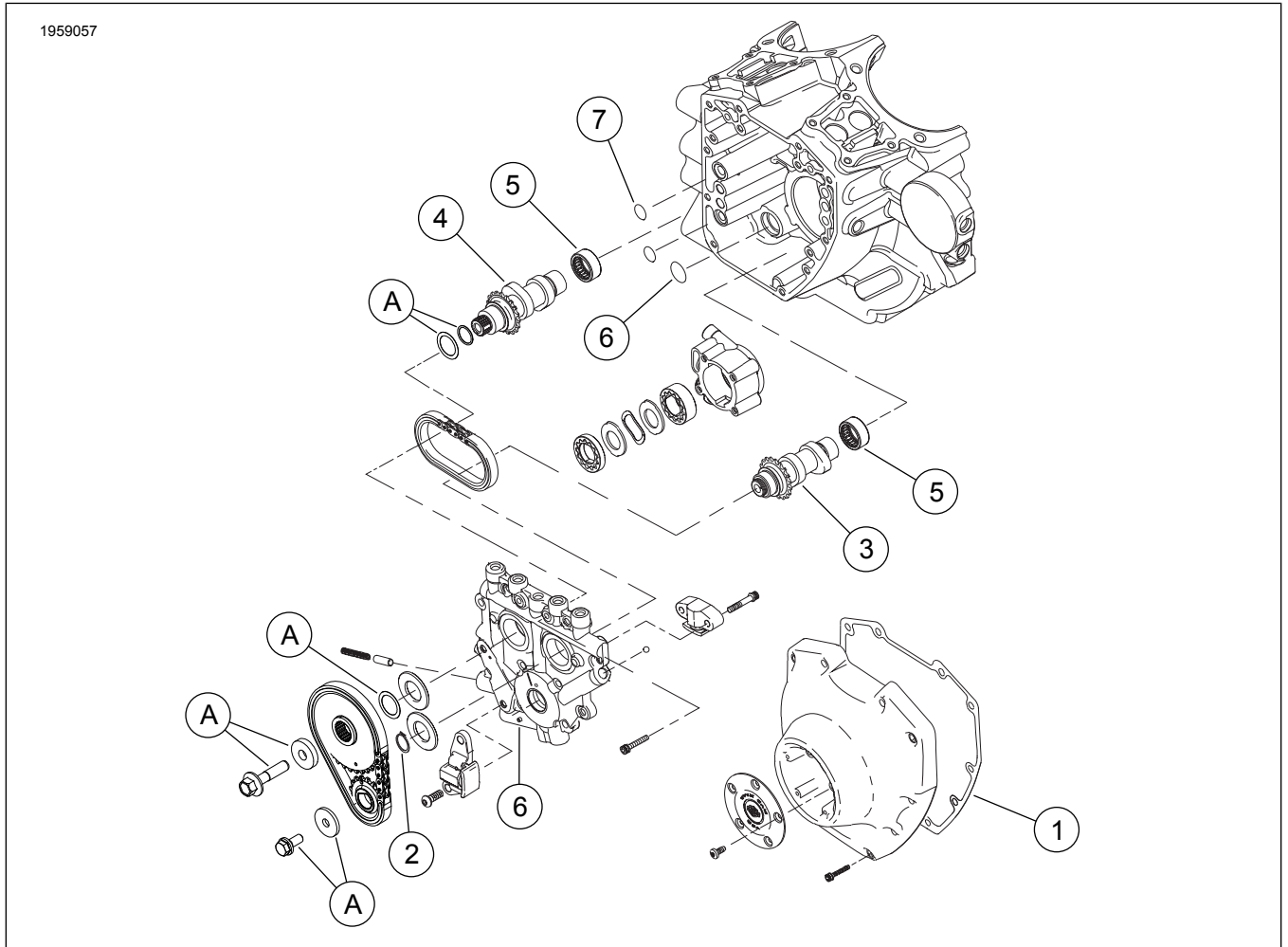
Gambar 3. Komponen Servis: Kit Stage 4 Screamin' Eagle Pro TC 103 (96 CI hingga 103 CI)
