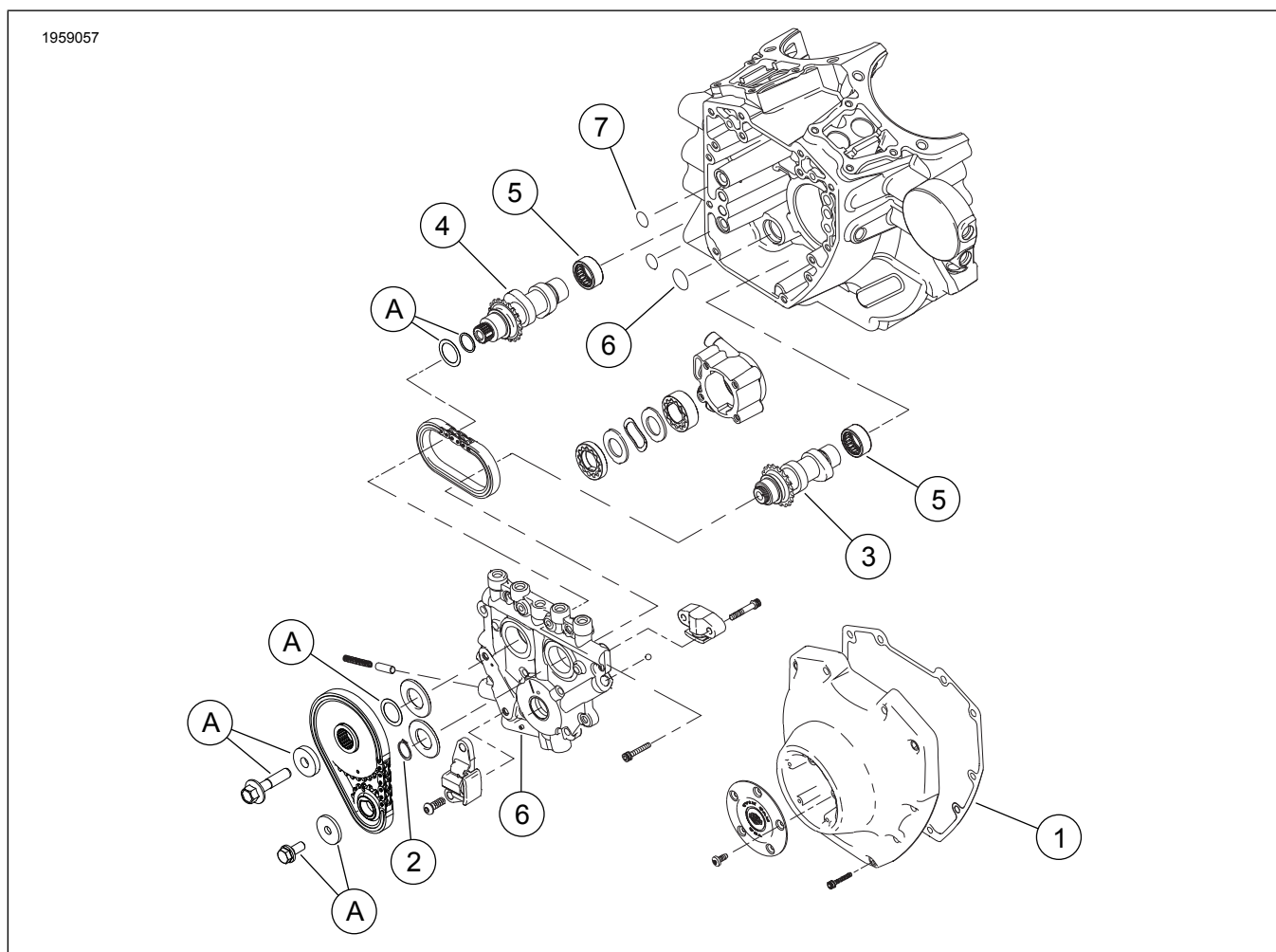
Figur 3. Reservdelar: Screamin' Eagle Pro TC 103 CI Steg 4-sats
