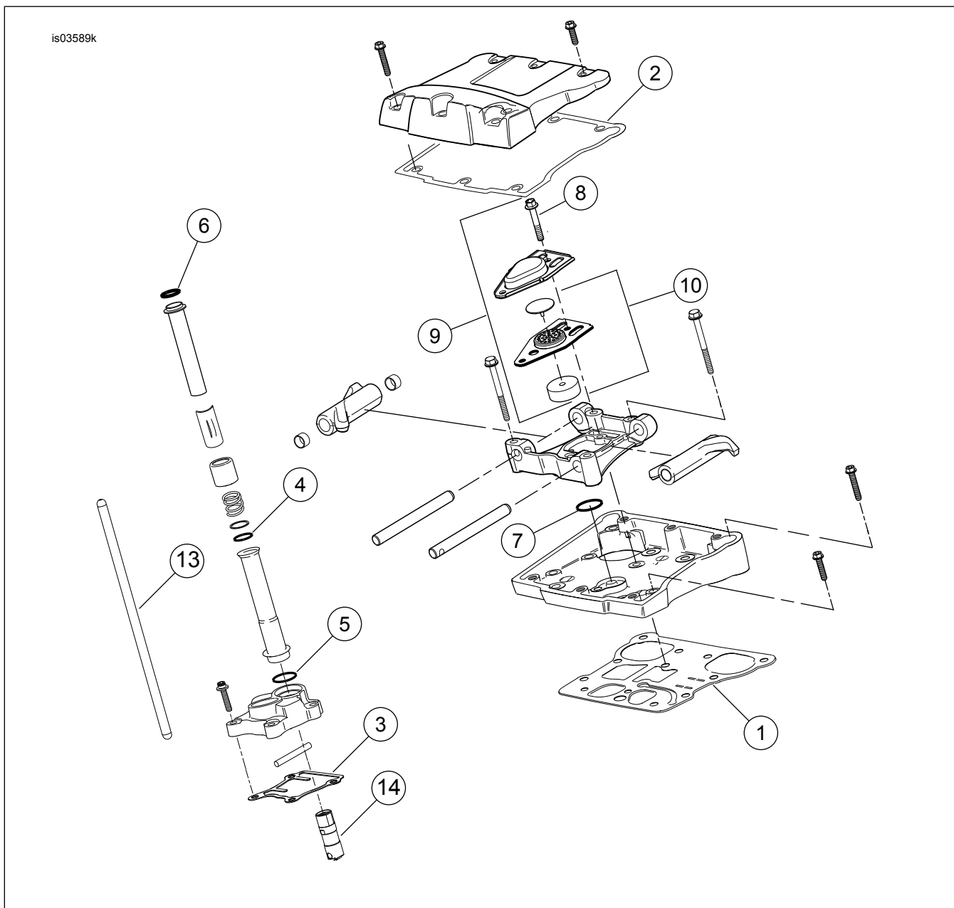
Figur 2. Servicedeler: Screamin' Eagle Pro TC 103 CI Stage 4-sett
