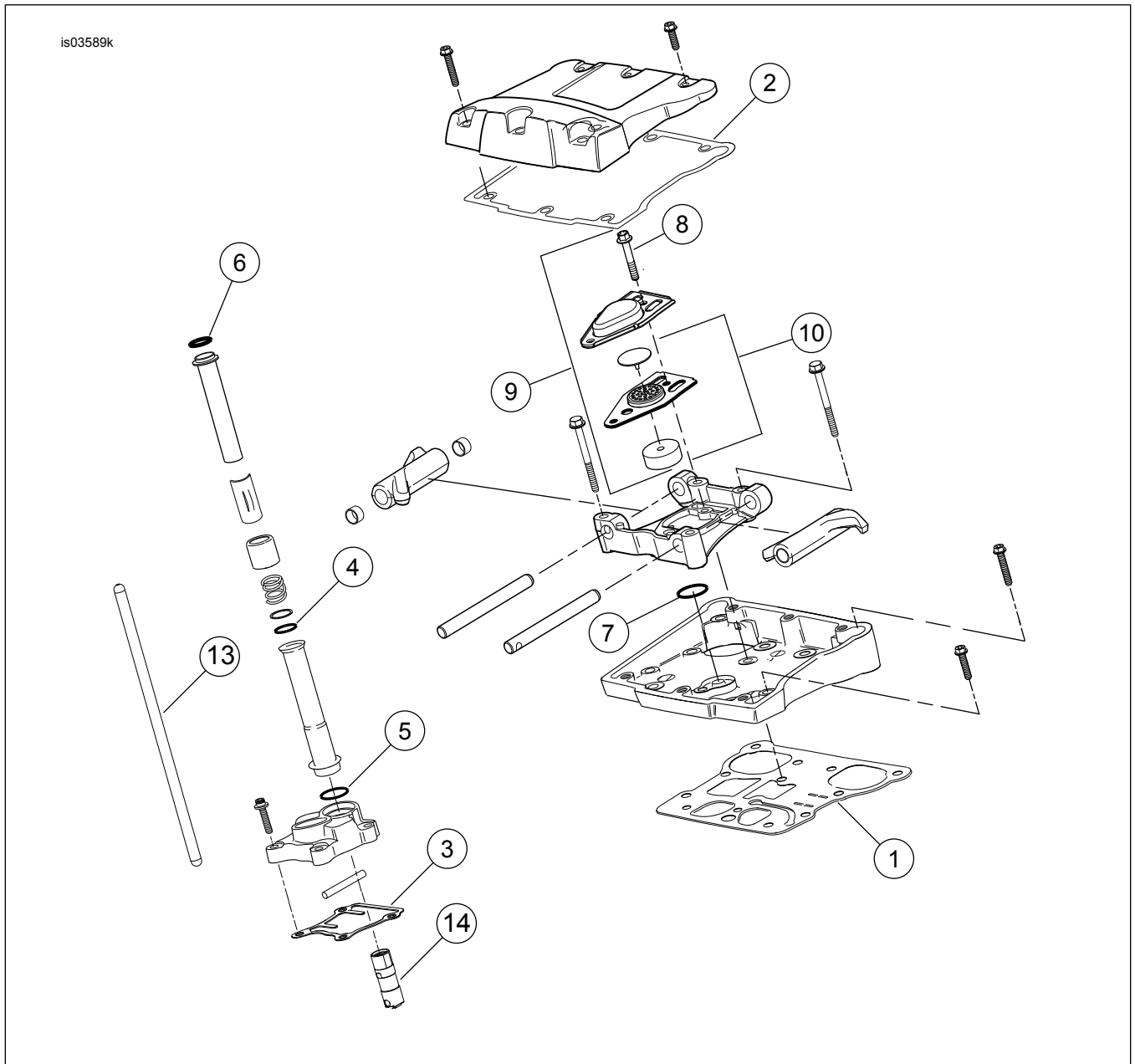
Figure 2. Service Parts: Screamin' Eagle Pro TC 103 CI Stage 4 Kit
