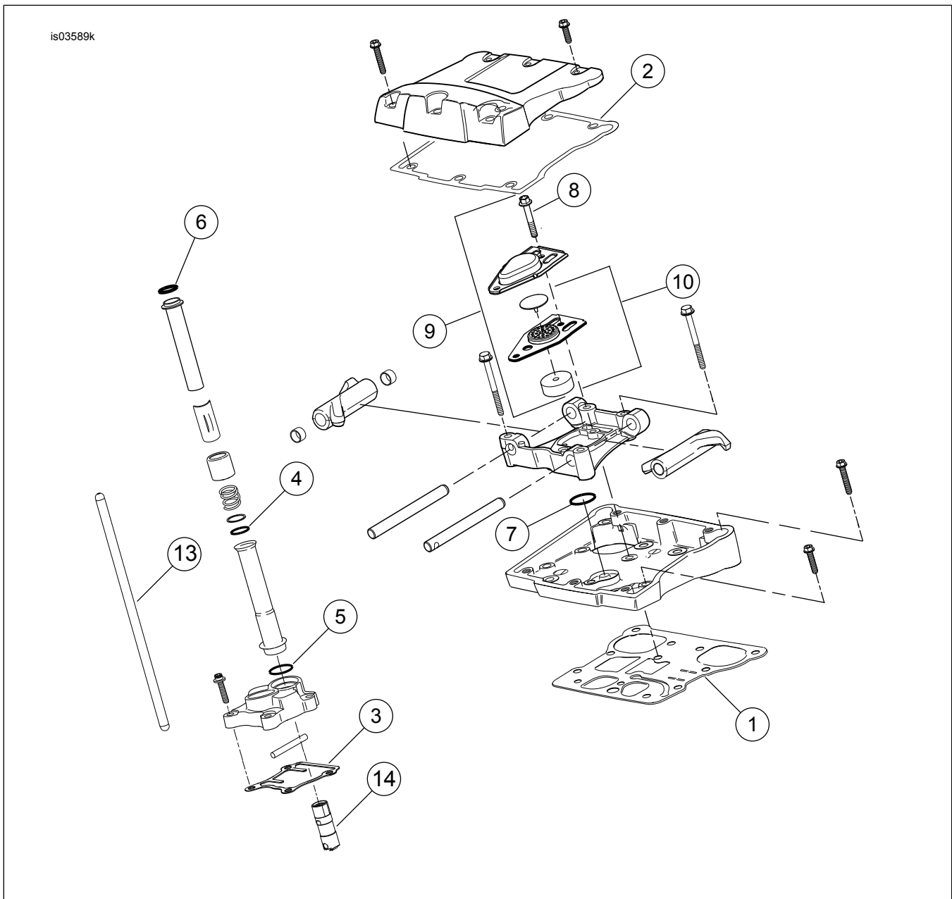
Gambar 2. Komponen Servis: Kit Stage Screamin' Eagle Pro TC 103 CI
