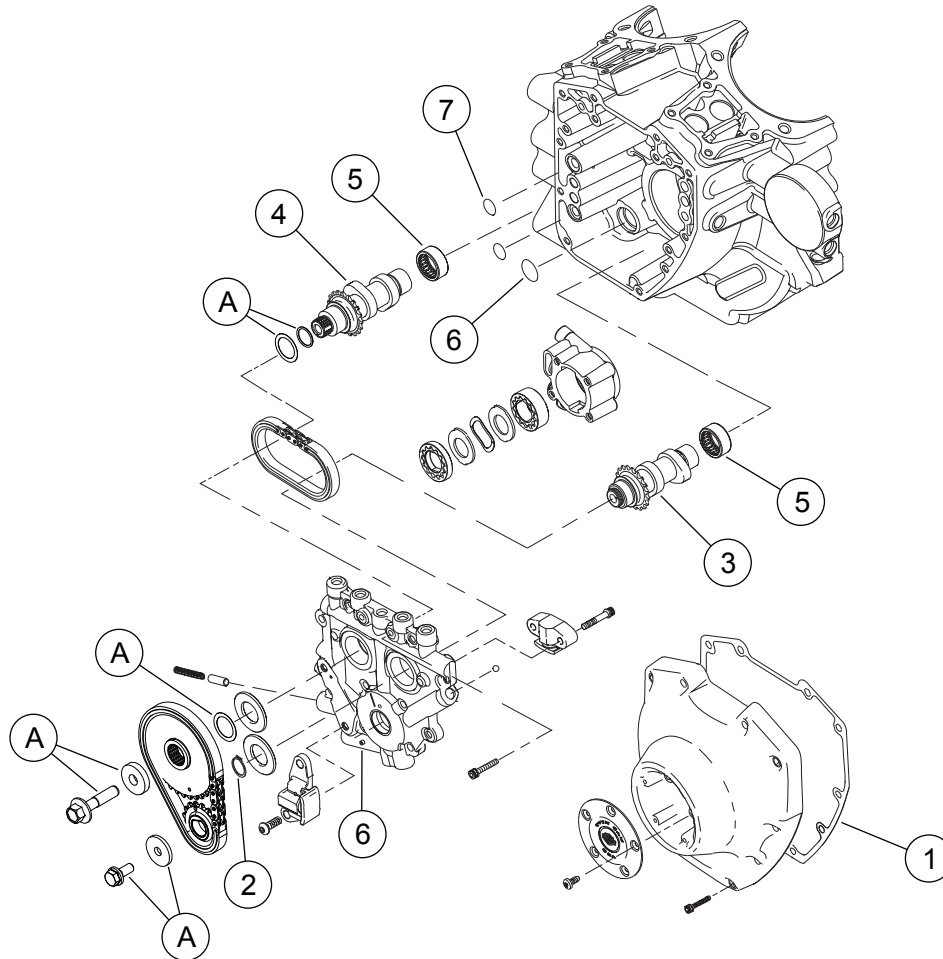
Gambar 3. Komponen Servis: Kit Stage Screamin' Eagle Pro TC 103 CI
