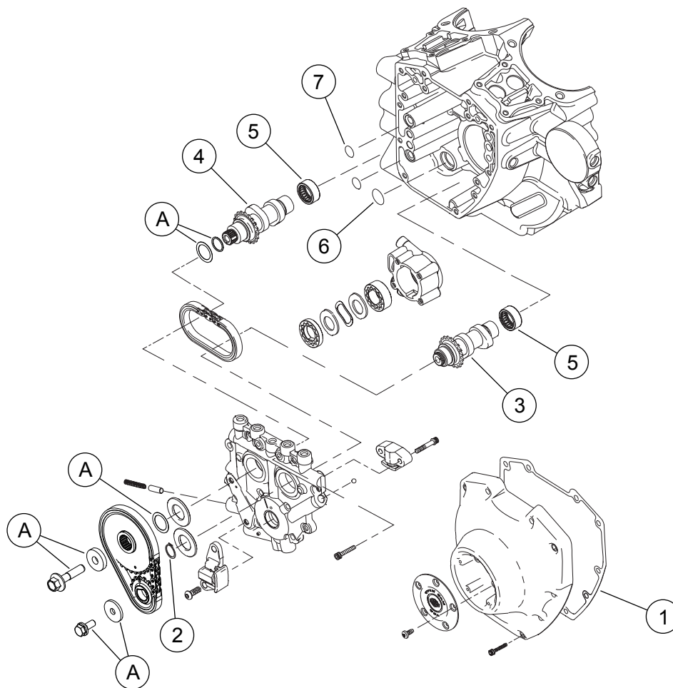
Figur 3. Reservdelar: Screamin' Eagle Pro TC 103 (1690 cc) Stage 4 Kit
