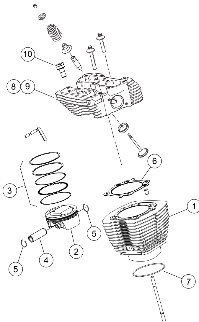
Figur 1. Reservdelar: Screamin' Eagle TC 103 (1690 cc) Stage 4 Kit
