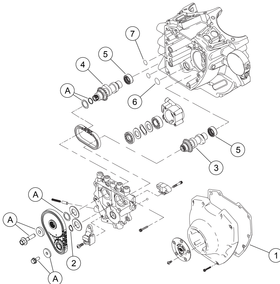
Figur 3. Servicedeler: Screamin' Eagle Pro TC 103 (1690 cc) nivå 4-sett
