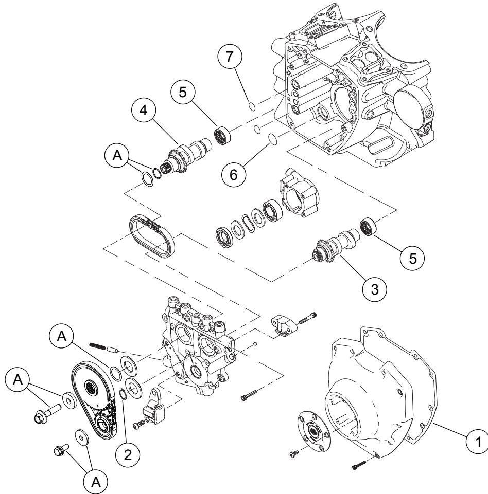
Figure 3. Service Parts: Screamin' Eagle Pro TC 103 (1690 cc) Stage 4 Kit
