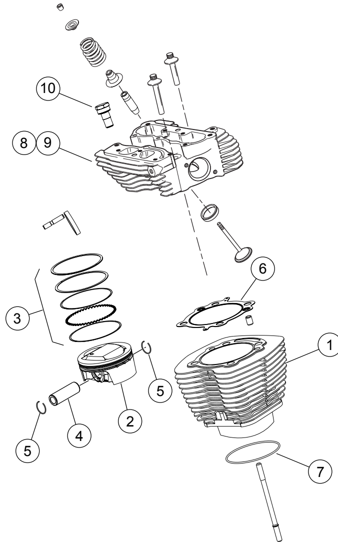
Figure 1. Service Parts: Screamin' Eagle TC 103 (1690 cc) Stage 4 Kit
