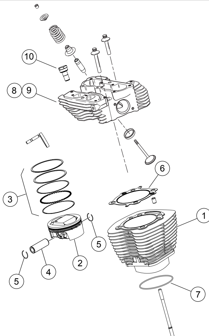
Figur 1. Reservedele: Screamin' Eagle TC 103 (1690 cc) Stage 4 Kit
