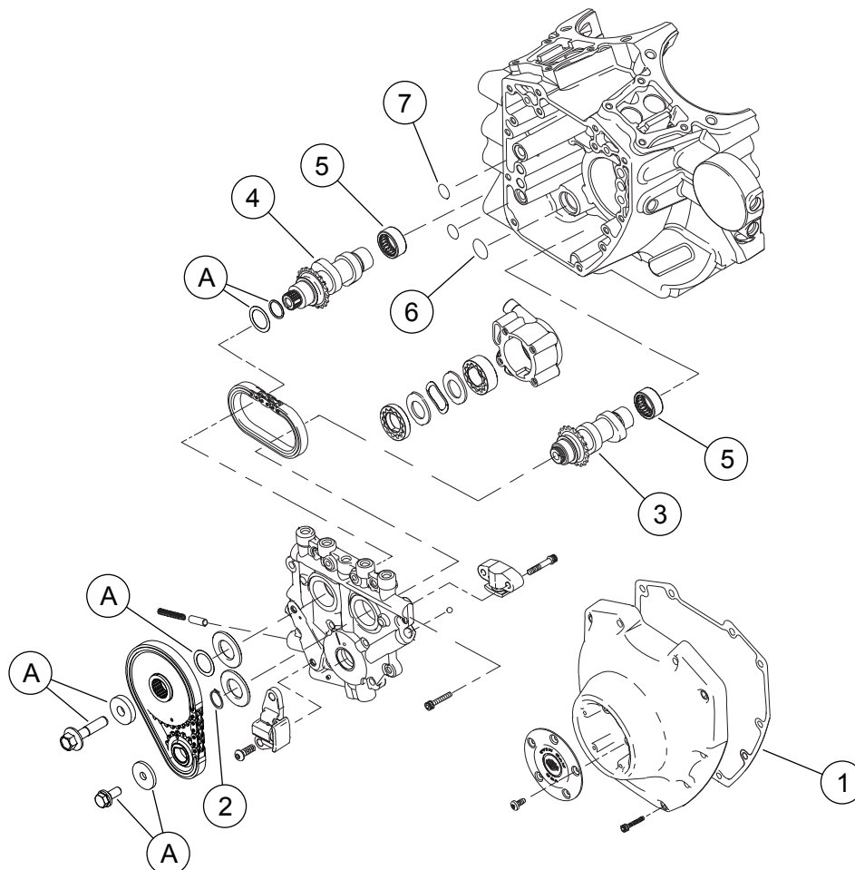
Gambar 3. Komponen Servis: Kit Screamin' Eagle Pro TC 103 (1690 cc) Stage 4
