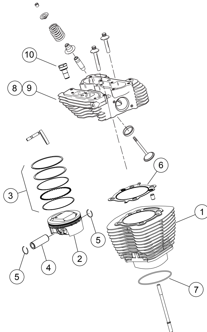
Gambar 1. Komponen Servis: Kit Screamin' Eagle TC 103 (1690 cc) Stage 4
