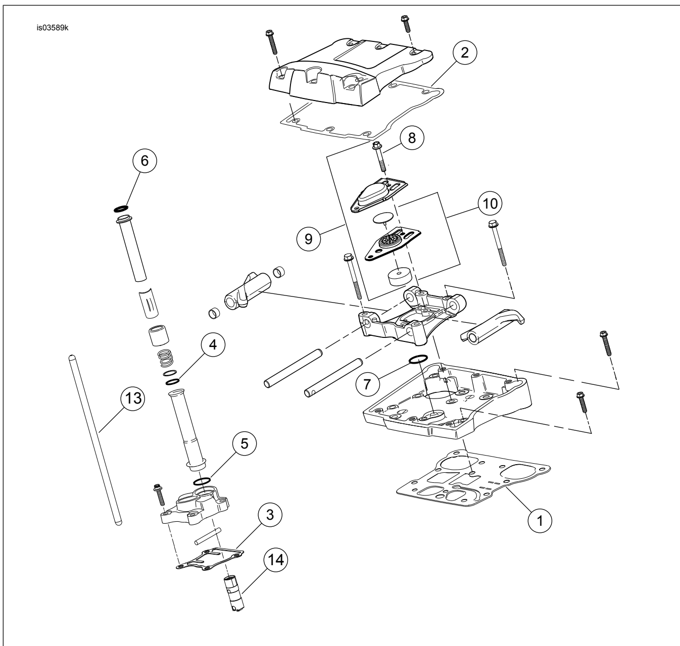
Gambar 2. Komponen Servis: Kit Screamin' Eagle TC 103 (1690 cc) Stage 4
