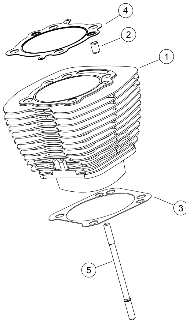
Figura 8. Cilindri bloc motor SE120R Screamin' Eagle Pro
